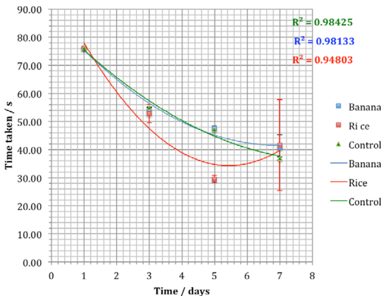
Time taken to decolorise KMnO 4 by extract of nectarines incubated with banana, rice or nothing. Error bars = ± 1 standard deviation
